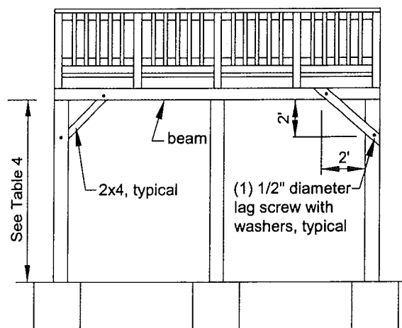
Figure 10. Diagonal Bracing.
